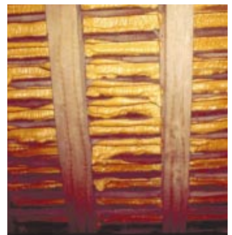
Figure 14 Sprayed foam used as a way of avoiding stripping a 'nail sick' roof and providing some insulation is NOT recommended good practice on a historic building. (Photograph courtesy of Kevin Stubbs, Bursledon Brickworks Conservation Centre)
